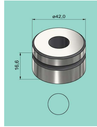
Rundmatrize APS 42
